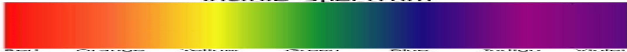
Visible Spectrum
