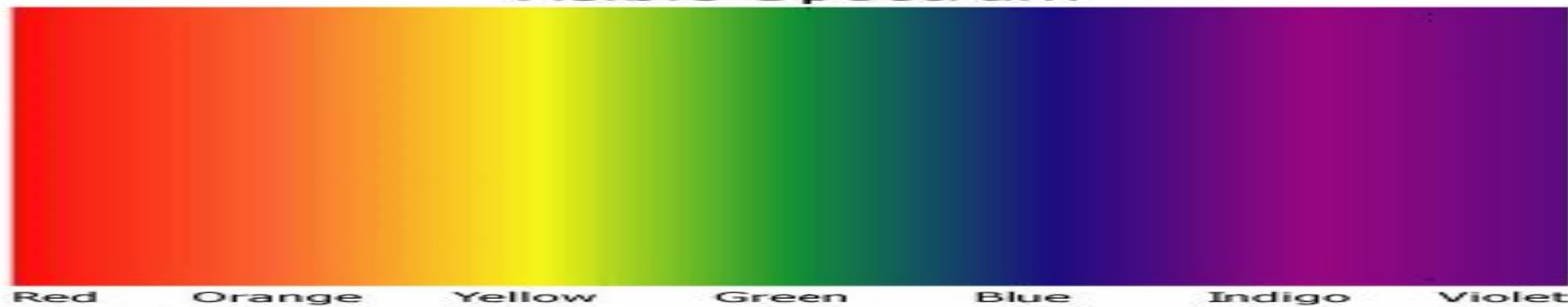
Visible Spectrum
